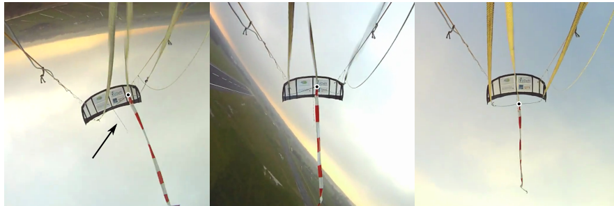
Fig. 15.4 Wing and bridle line system during a downloop figure eight maneuver performing a right turn (left) and following straight flight diagonally upwards (center) and during retraction of the kite (right). Video stills taken from the kite control unit (24 November 2010)
