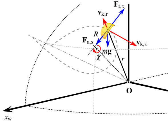
Fig. 15.3 Kite performing a left turn ( \dot{\chi} > 0 ) while flying a downloop figure eight maneuver and generating traction power ( v_{k,r} > 0 ). Only one half of the maneuver is displayed. The dash-dotted line passing through the center of the turn is the turning axis, while the corresponding turn radius is denoted as R and the non-dimensional turning radius is defined as \rho = R/r
