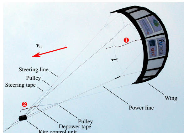
Fig. 15.1 Kite system consisting of a flexible membrane wing with 25 m 2 total surface area, a bridle line system to transfer the aerodynamic load and a suspended, remote-controlled cable robot (kite control unit) [18]. For this specific flight a piece of barricade tape ① is attached to the rear end of the center strut of the kite and another piece ② is attached to the end of the depower tape to indicate the direction of the apparent wind (24 November 2010)
